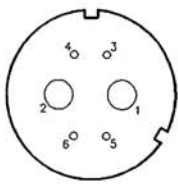
2 EACH #0 4 EACH #12
