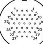
37 EACH #16
