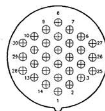
30 EACH #16
