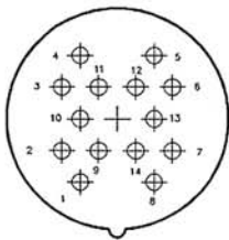
14 EACH #16
