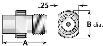
Figure 1 (Straight jack, direct solder)
