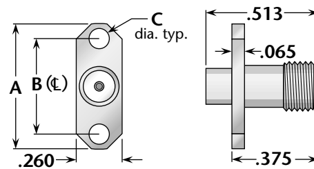
Figure 4 (2-hole flange, direct solder)
